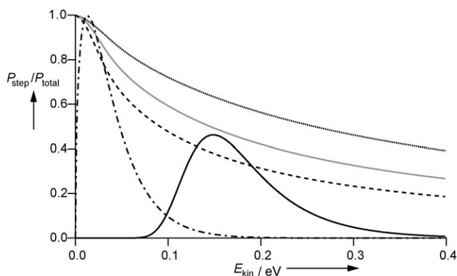
Figure 2. Fraction of reactivity at the step sites versus kinetic energy. •••• Pt(211), — Pt(533), ---- Pt(755). Maxwell-Boltzmann distributions for gas temperatures of 300 (---) and 1000 K (—) are also shown. See text for details.
